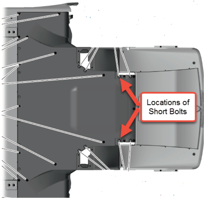
Figure 2: Location of the two (2) short bolts indication
